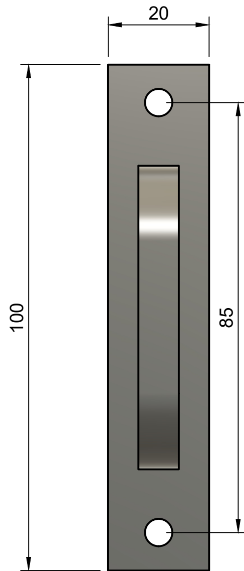
Lock Body
